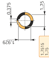
Hollow output shaft
